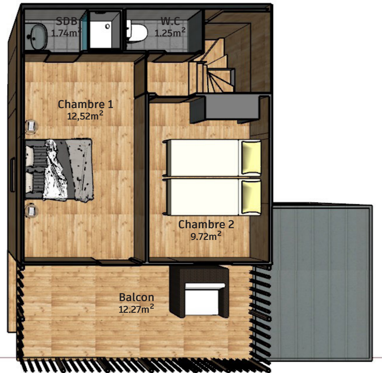
PLAN R+1
